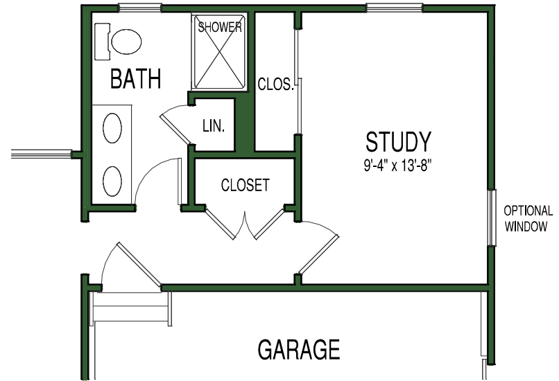
OPTIONAL 3'-0" REAR EXPANSION TO STUDY AND BATH WITH OPTIONAL SHOWER
