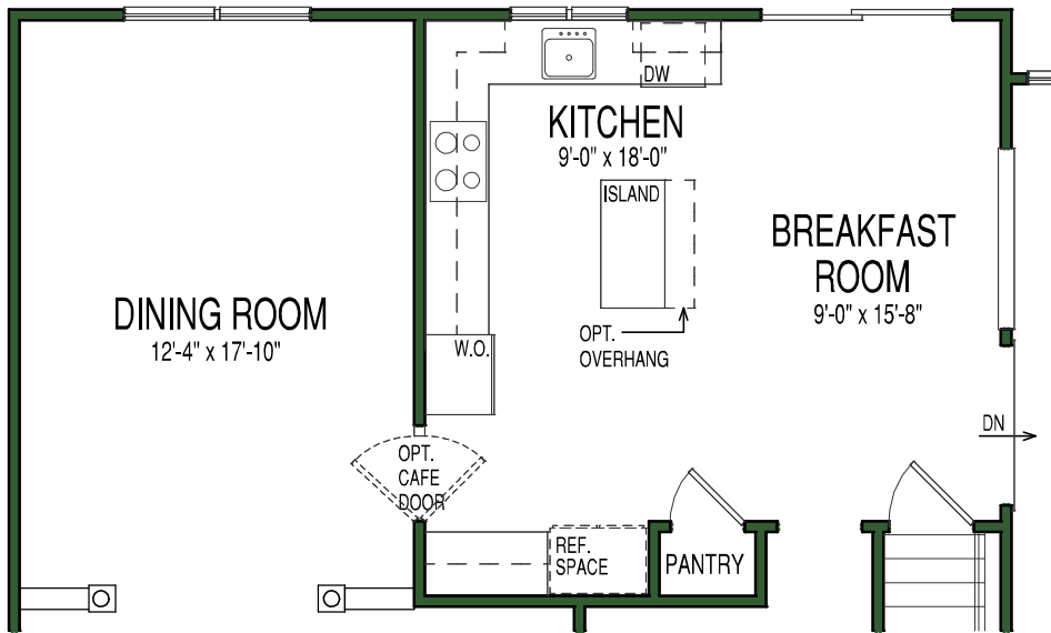
OPTIONAL 2'-0" REAR EXPANSION TO DINING ROOM, KITCHEN AND BREAKFAST ROOM
