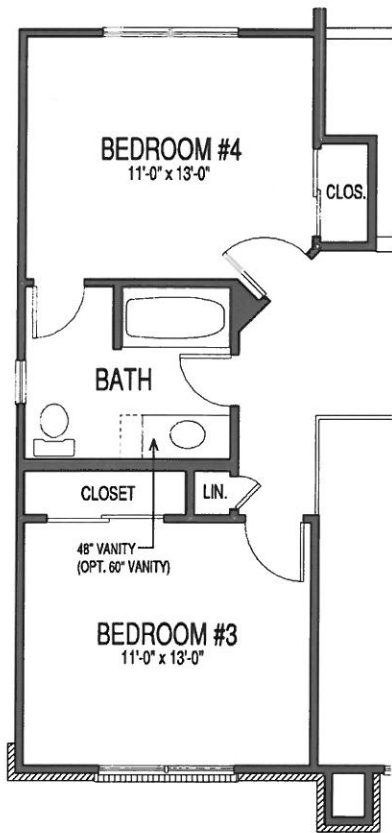
OPTIONAL SHARED PRINCESS BATH (AVAILABLE WITH LOFT OR 5TH BR OPTION ONLY)
