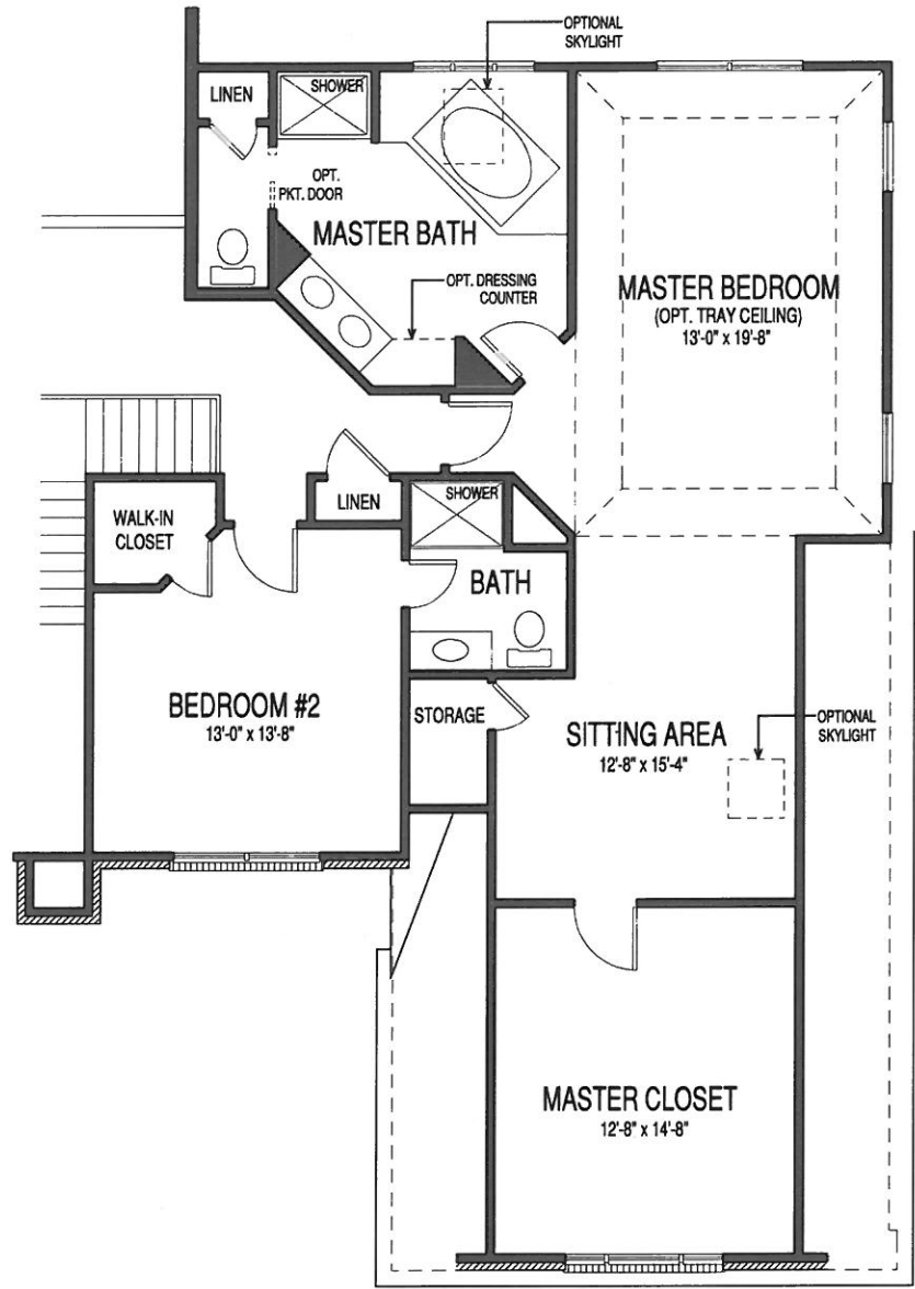
OPTIONAL SITTING AREA AND MASTER CLOSET LAYOUT WITH PRINCESS SUITE FOR BEDROOM #2
