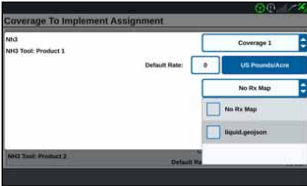
FIGURE 34. Coverage to Implement Assignment
