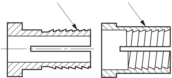
STYLE 2: A 7Z39-series Single-Ended
