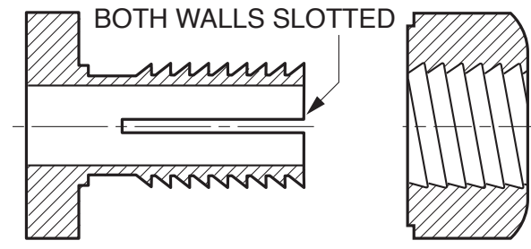
STYLE 3: Shaftloc® M-Type
