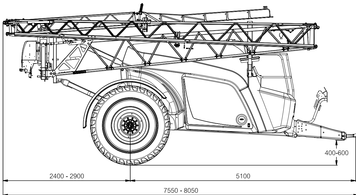
Ixtrack T4 dimensions
