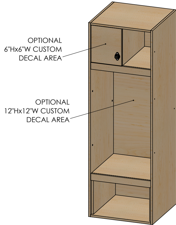
LOCKER SHOWN WITHOUT OPTIONAL 4" HIGH TOE KICK BASE
