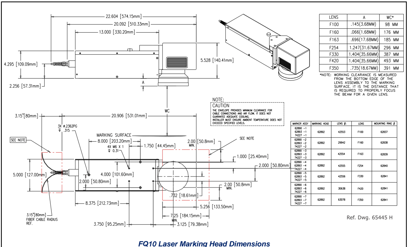
FQ10 Laser Marking Head Dimensions
