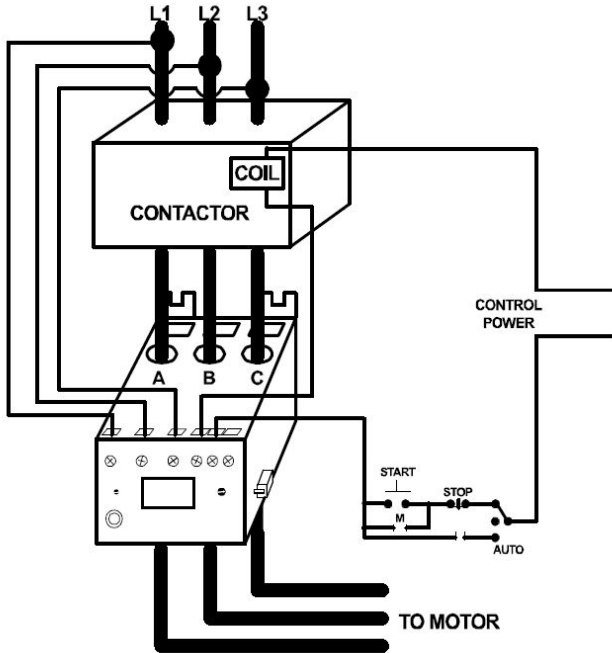
Figure 2. Typical wiring diagram of a 777 PumpSaver®
