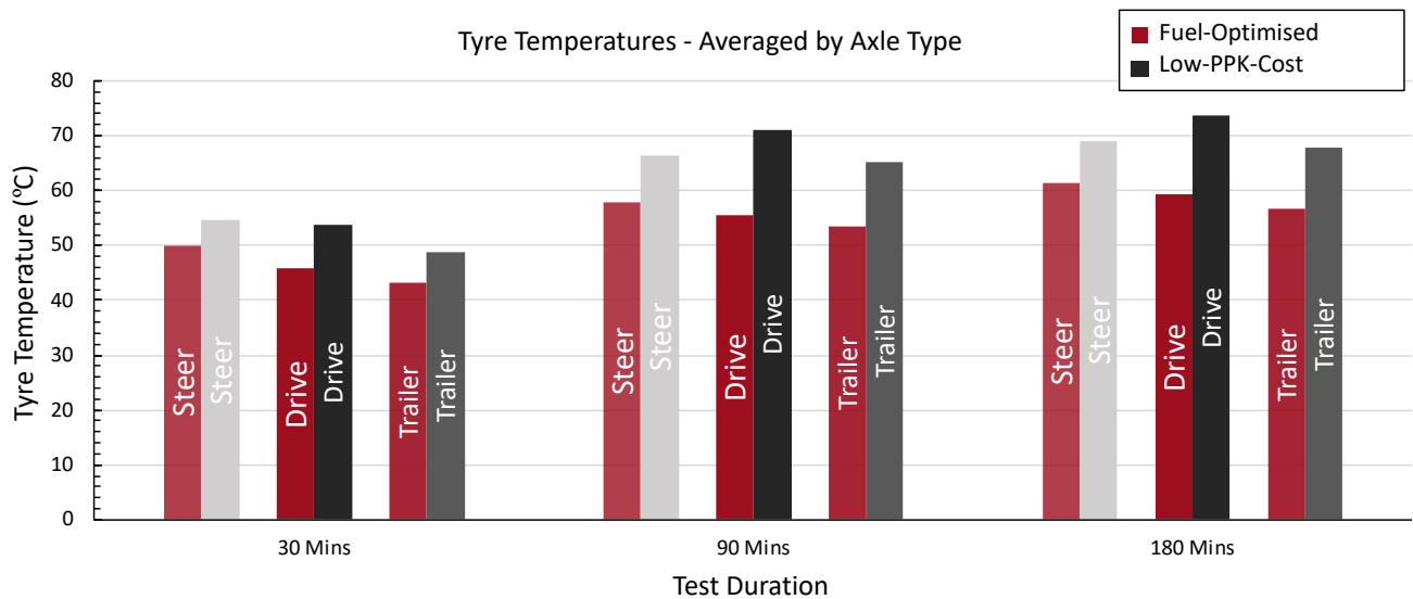
Figure 1. Axle-by-axle comparison of the final temperature of the low-PPK-cost and fuel-optimised tyre policies after testing period.
