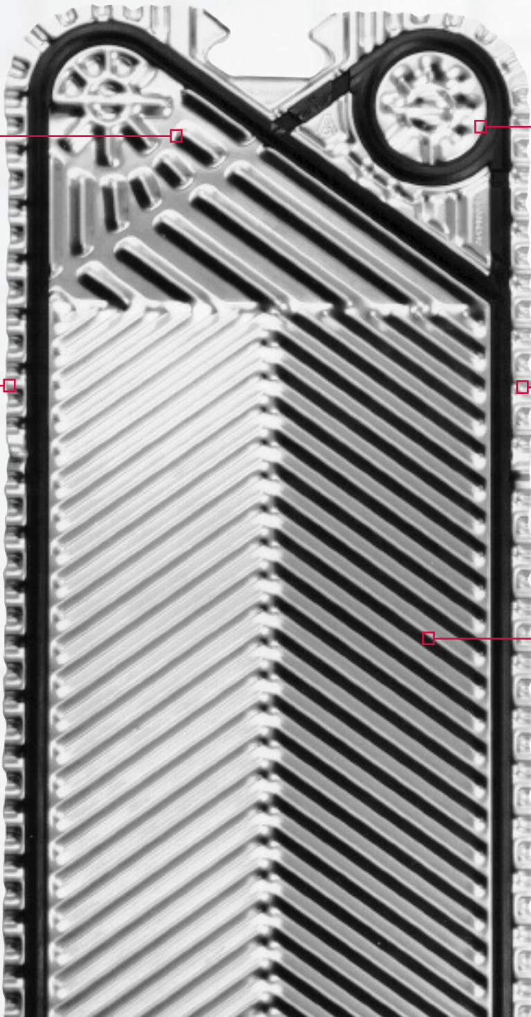
Partially relieved gasket groove reduces product to gasket contact area
