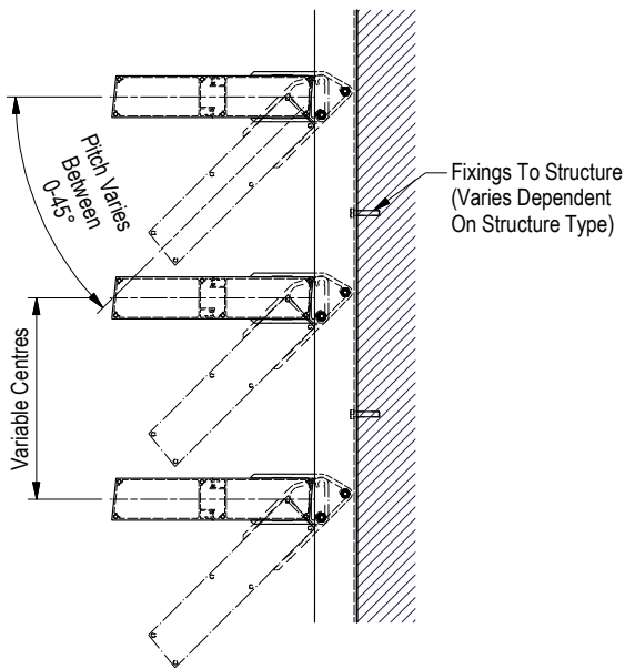
SECTIONED VIEW
