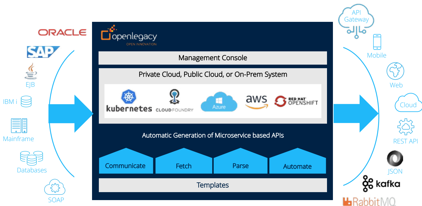
OpenLegacy platform's overall architecture showing its major functionality, the potential inputs, and how it outputs to a number of different types of systems.
