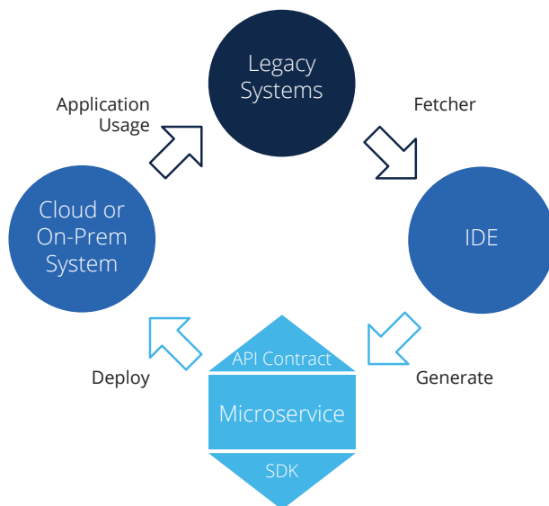
OpenLegacy's design-time and run-time processes for building and using microservice-based APIs for legacy systems
