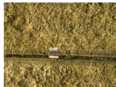
Weld Seam Corrosion Leak
