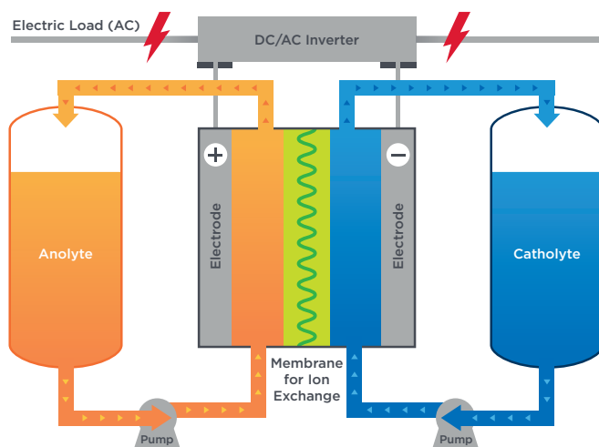
FIGURE 1: Diagram of flow battery process. Source: Summary of 2017 NASA Workshop on Assessment of Advanced Battery Technologies for Aerospace Applications.
