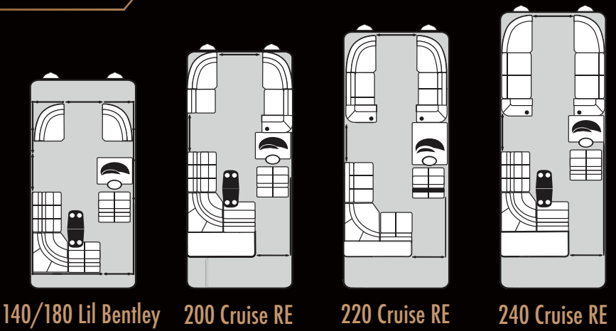
» Floor Plans
