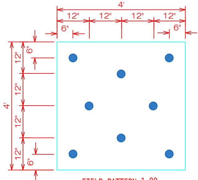
FIELD PATTERN 1-90 4' X 8' = 16 PER BOARD 4' X 4' = 8 PER BOARD
