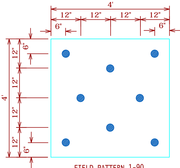
FIELD PATTERN 1-90 4' X 8' = 16 PER BOARD 4' X 4' = 8 PER BOARD
