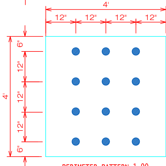
PERIMETER PATTERN 1-90 NON-HURRICANE ZONE 4' X 8' = 24 PER BOARD 4' X 4' = 12 PER BOARD
