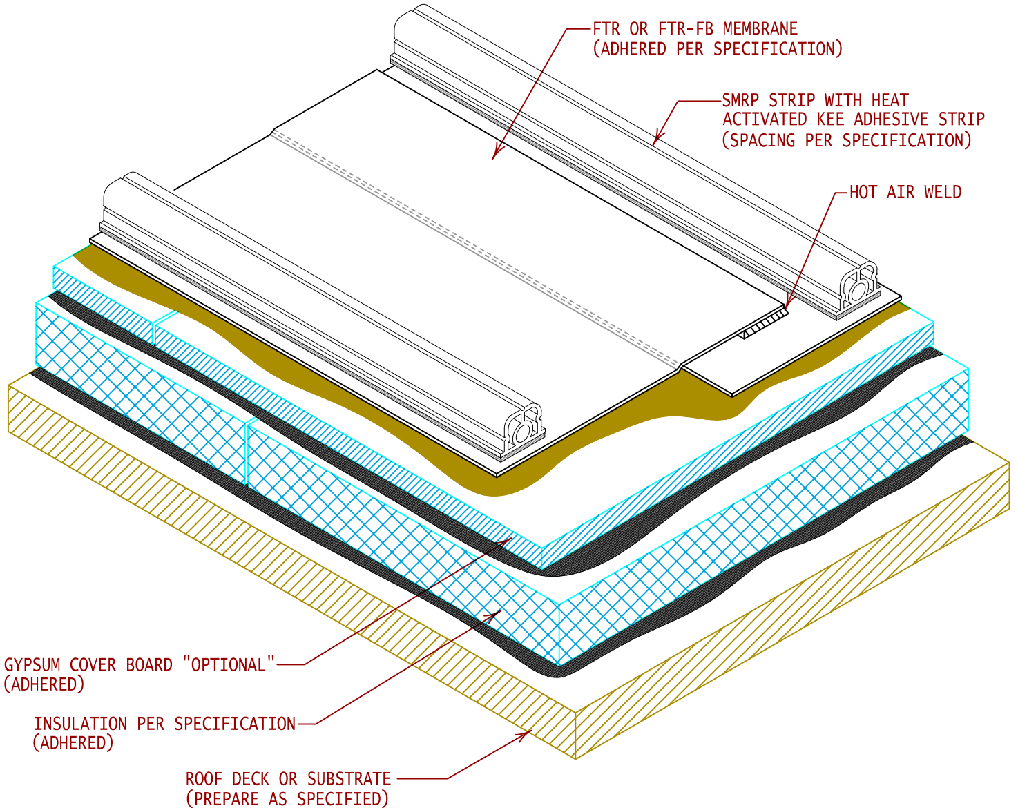
SMRP SECTION VIEW
