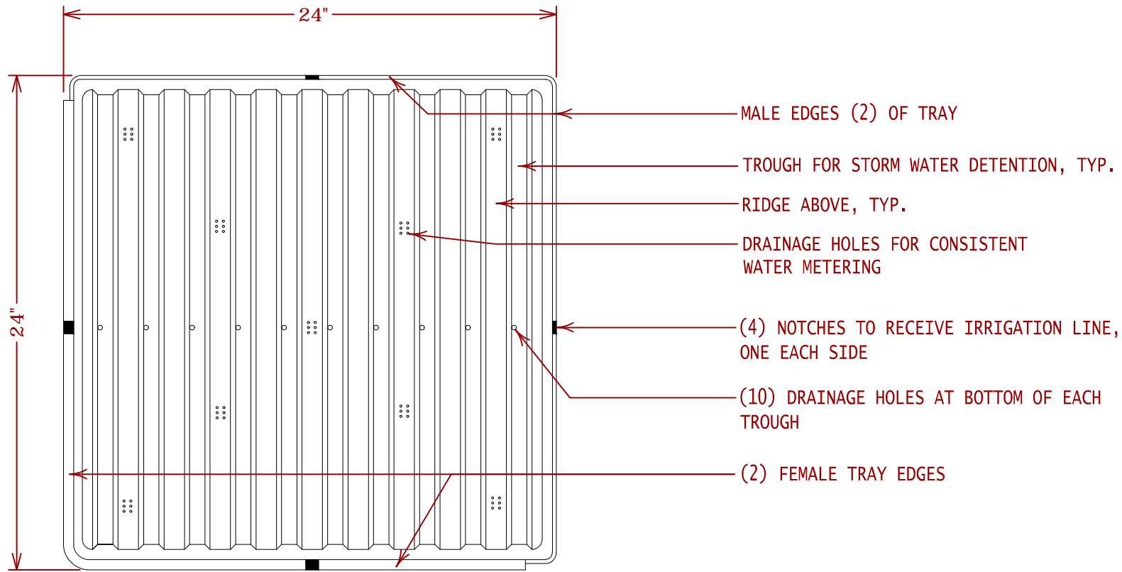
PLAN VIEW
