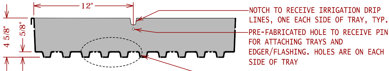
SECTION-ELEVATION
