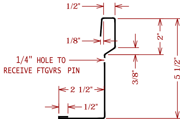
A FTGVRS EDGING PART NO. - EDG-001
