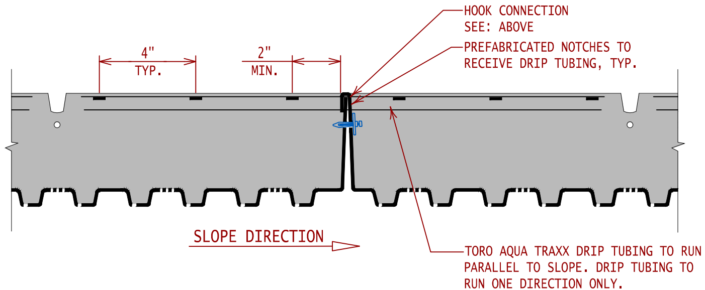
HOOK CONNECTION SCALE: NTS
