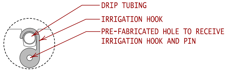
HOOK CONNECTION SCALE: NTS
