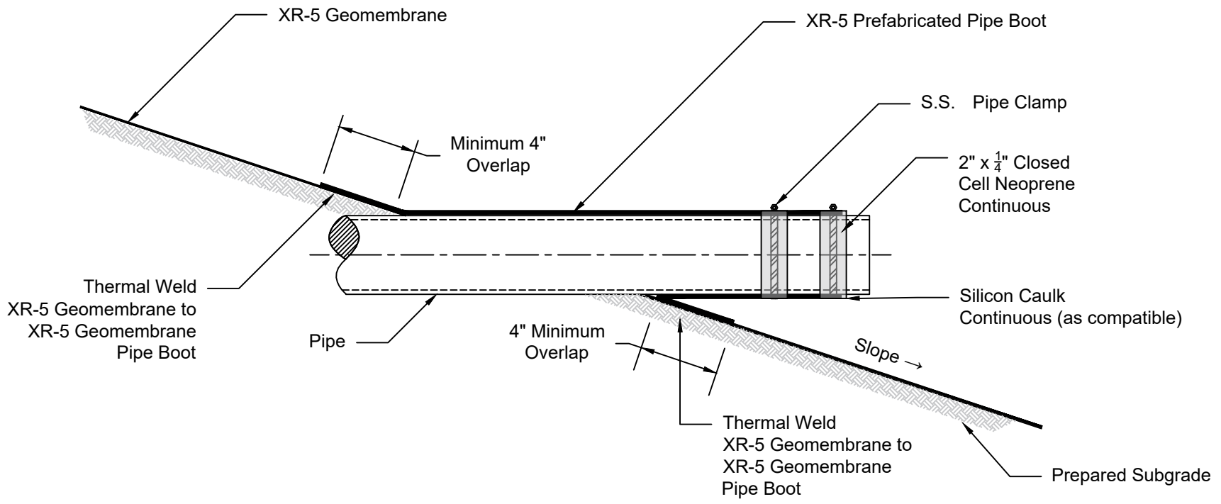
Cross Section
