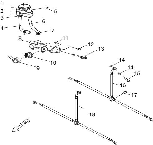
D-16:BRAKE LINES/MASTER CYLINDER
