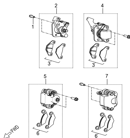
D-19:REAR BRAKE CALIPER
