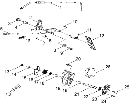
D-14:THROTTLE
