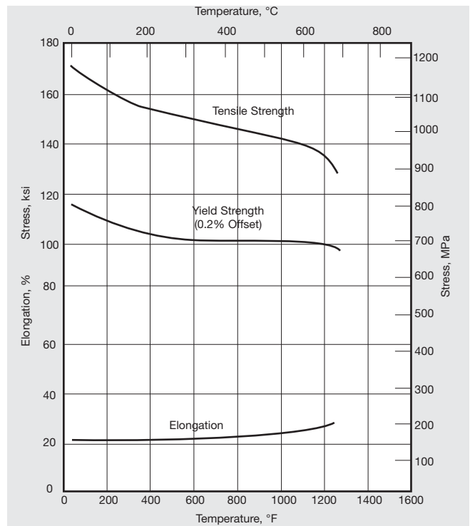
Figure 1. Tensile properties at high temperatures of solution-annealed and aged INCOLOY alloy 925.
