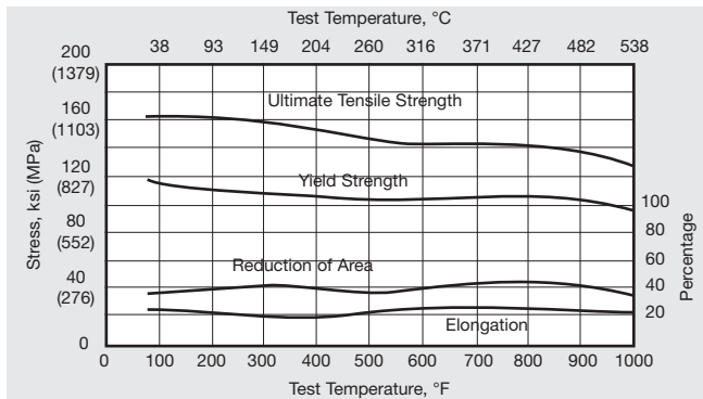
Figure 7. INCOLOY alloy 925 GTA weld data. Pre-weld treatment: anneal. Post-weld treatment: anneal plus age. Anneal = 1900°F (1040°C)/1 h/AC. Age = 1365°F (740°C)/6-9 h/FC to 1150°F (621°C) ±15°F (8°C) for a total aging time of 18 h.
