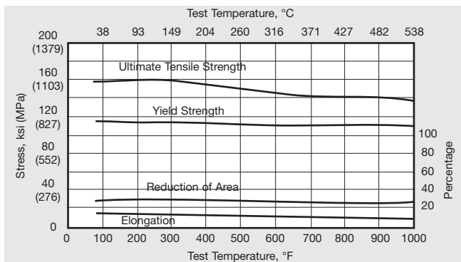
Figure 9. INCOLOY alloy 925 GTA weld data. Pre-weld treatment: age. Post-weld treatment: age. Anneal = 1900°F (1040°C)/1 h/AC. Age = 1365°F (740°C)/6-9 h/FC to 1150°F (621°C) ±15°F (8°C) for a total aging time of 18 h.
