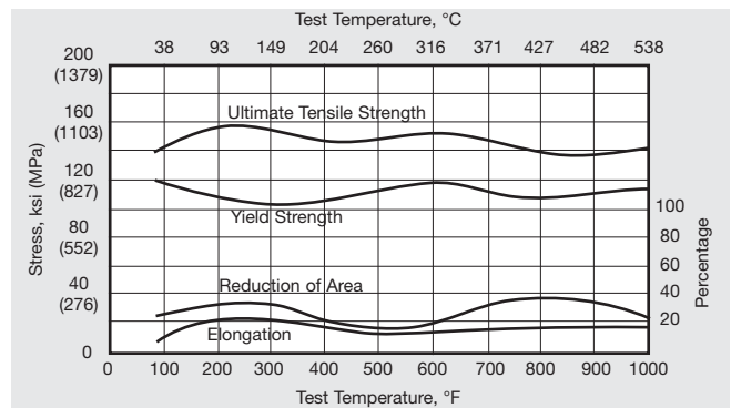
Figure 10. INCOLOY alloy 925 GMA weld data. Pre-weld treatment: anneal. Post-weld treatment: anneal plus age. Anneal = 1900°F (1040°C)/1 h/AC. Age = 1365°F (740°C)/6-9 h/FC to 1150°F (621°C) ±15°F (8°C) for a total aging time of 18 h.
