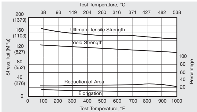
Figure 11. INCOLOY alloy 925 GMA weld data. Pre-weld treatment: anneal. Post-weld treatment: age. Anneal = 1900°F (1040°C)/1 h/AC. Age = 1365°F (740°C)/6-9 h/FC to 1150°F (621°C) ±15°F (8°C) for a total aging time of 18 h.
