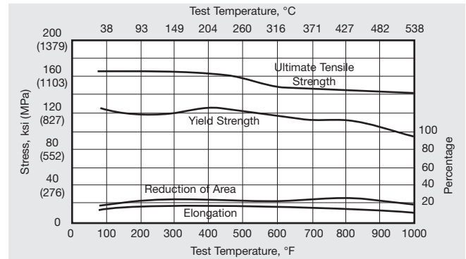
Figure 12. INCOLOY alloy 925 GMA weld data. Pre-weld treatment: age. Post-weld treatment: age. Anneal = 1900°F (1040°C)/1 h/AC. Age = 1365°F (740°C)/6-9 h/FC to 1150°F (621°C) ±15°F (8°C) for a total aging time of 18 h.
