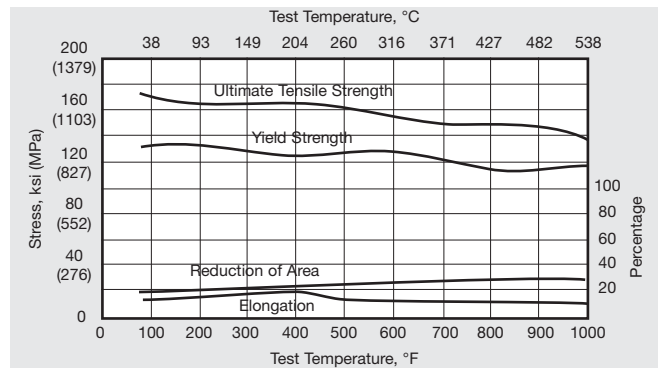
Figure 8. INCOLOY alloy 925 GTA weld data. Pre-weld treatment: anneal. Post-weld treatment: anneal. Anneal = 1900°F (1040°C)/1 h/AC. Age = 1365°F (740°C)/6-9 h/FC to 1150°F (621°C) ±15°F (8°C) for a total aging time of 18 h.
