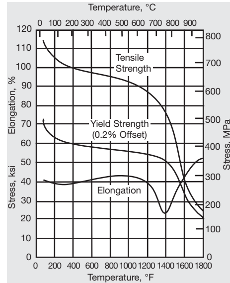
Figure 13. High-temperature tensile properties of all-weld metal specimens from gas-metal-arc welds made with INCONEL Filler Metal 617.
