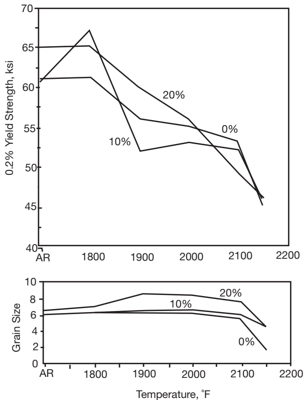
Figure 15. Effect of cold work and subsequent annealing temperature (annealed for 1 hour and air cooled) on the yield strength and grain size of alloy 617.
