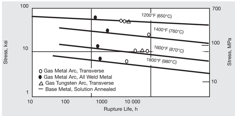
Figure 14. Rupture-strength comparison for base metal and joints welded with INCONEL Filler Metal 617.
