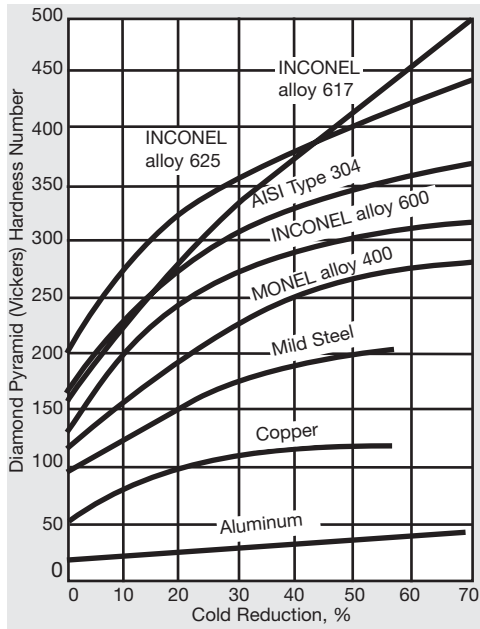
Figure 12. Effect of cold reduction on hardness.
