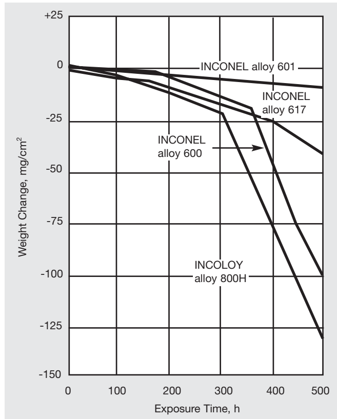
Figure 10. Resistance to oxidation at 2100°F (1150°C). Samples were exposed to temperature in 50-h cycles.
