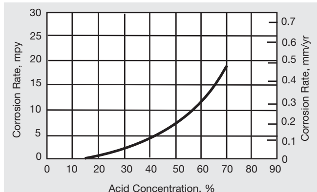
Figure 11. Corrosion rates in boiling nitric acid.
