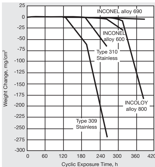
Figure 6. Cyclic oxidation resistance at 1800°F (980°C) of specimens coated with sodium sulfate. Cycles consisted of 15 min heating and 5 min cooling in air.
