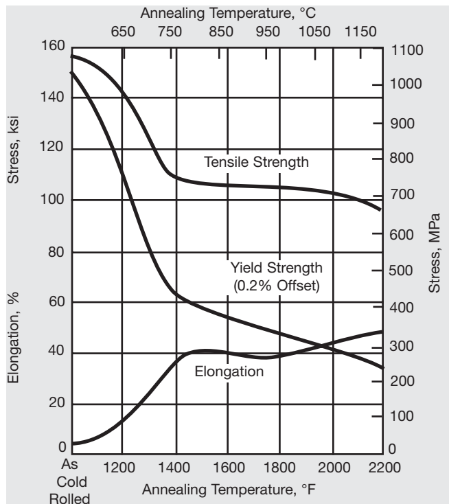
Figure 8. Effect of annealing temperature on tensile properties of cold-rolled sheet.
