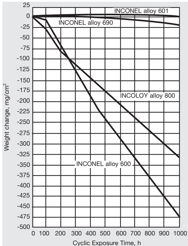
Figure 5. Cyclic oxidation resistance at 2000°F (1095°C). Cycles consisted of 15 min heating and 5 min cooling in air.
