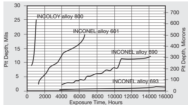
Figure 9. Maximum pitting depth as a function of time after exposure in CO-20% H 2 at 1150°F (621°C) for 120-grit ground samples.
