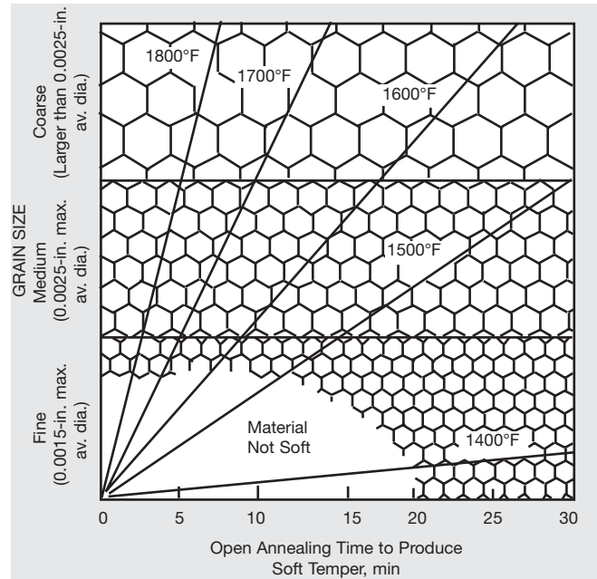
Figure 15. Approximate time required at various temperatures to produce different grain sizes in MONEL alloy 400 cold-rolled strip by open annealing.
