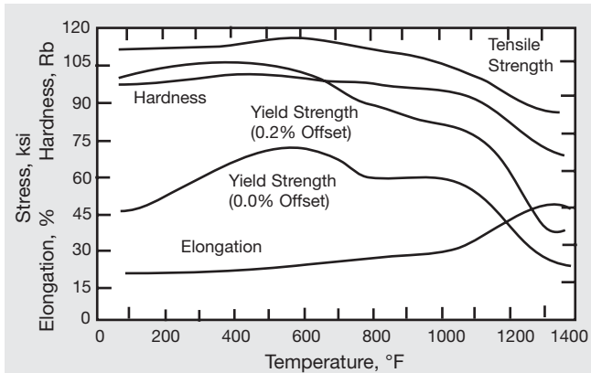
Figure 12. Effect of annealing (3 hr) on room-temperature properties of MONEL alloy 400 cold-drawn rod.
