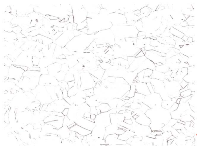
Figure 11. Longitudinal section of cold-drawn MONEL alloy 400 rod. Etchant: Sodium cyanide--ammonium persulfate. 100X.
