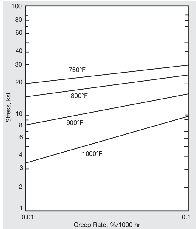
Figure 7. Creep properties of cold-drawn annealed (1500°F/3 hr) MONEL alloy 400.
