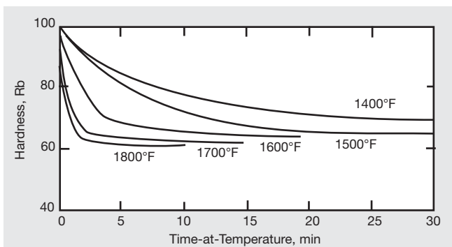
Figure 14. Approximate time required at various temperatures to produce different hardness levels in MONEL alloy 400 cold-rolled strip by open annealing.
