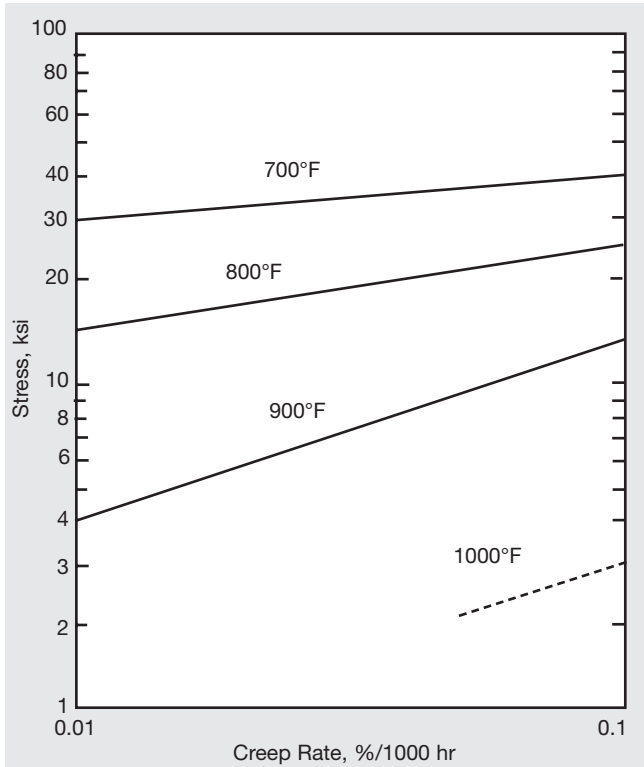
Figure 6. Creep properties of hot-rolled MONEL alloy 400.
