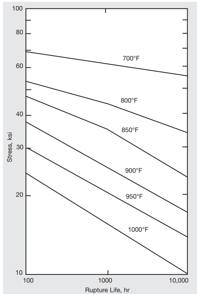
Figure 10. Rupture properties of cold-drawn, stress-relieved (1100°F/8 hr) MONEL alloy 400.
