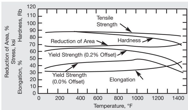
Figure 13. Effect of annealing (3 hr) on room-temperature properties of hot-rolled MONEL alloy 400 plate. At 1470°F, material is fully annealed. (Hardness converted from BHN.).
