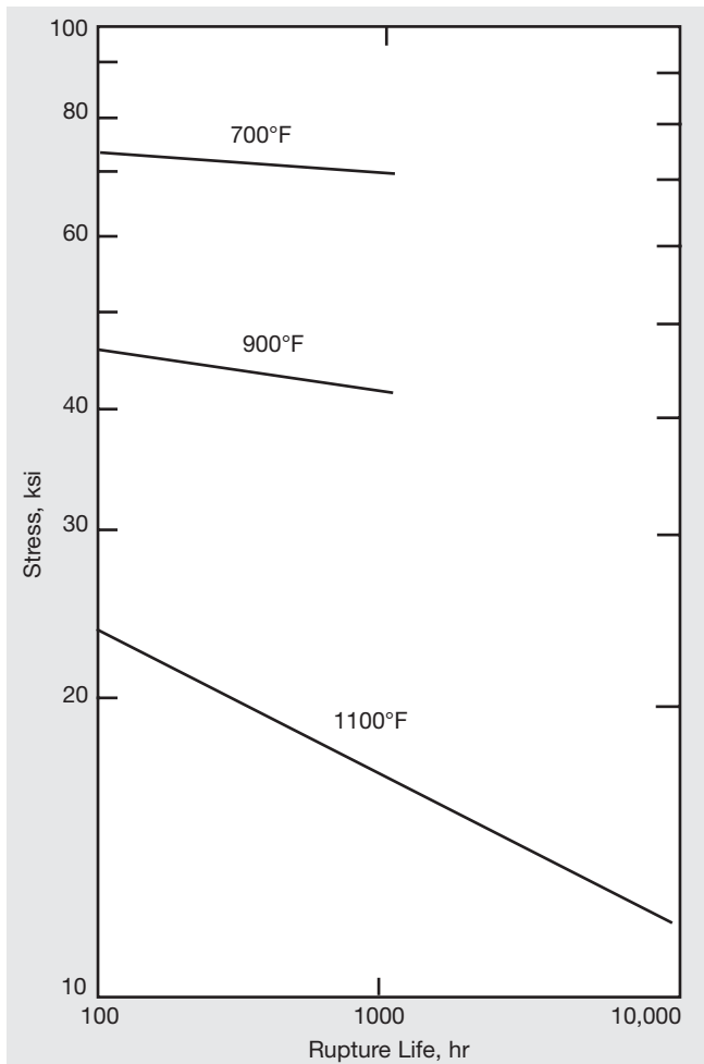
Figure 9. Rupture properties of cold-drawn annealed (1500°F/30 min) MONEL alloy 400.
