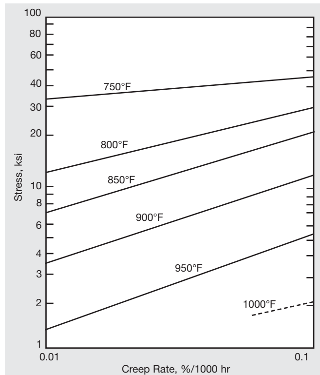
Figure 8. Creep properties of 20% cold-drawn stress-relieved (1000°F/8 hr) MONEL alloy 400.
