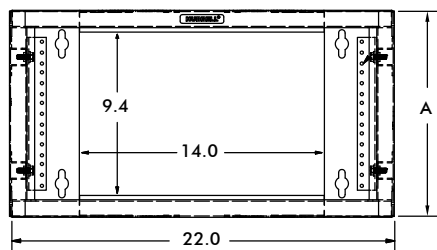
FRONT VIEW (WITHOUT DOOR)
