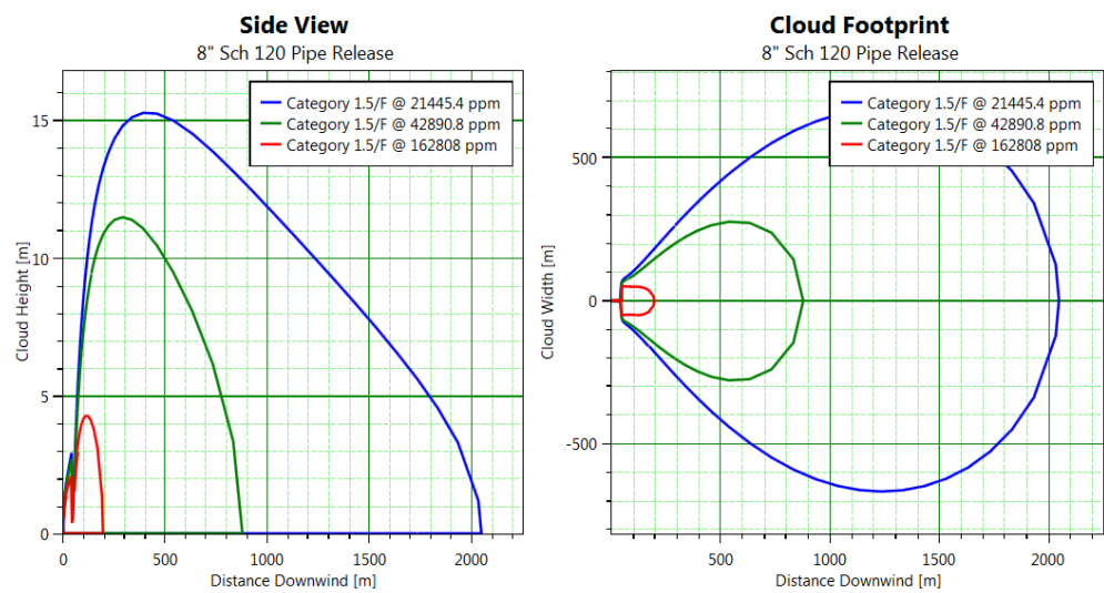
Figure 6: Horizontal release of high pressure LNG in PHAST
