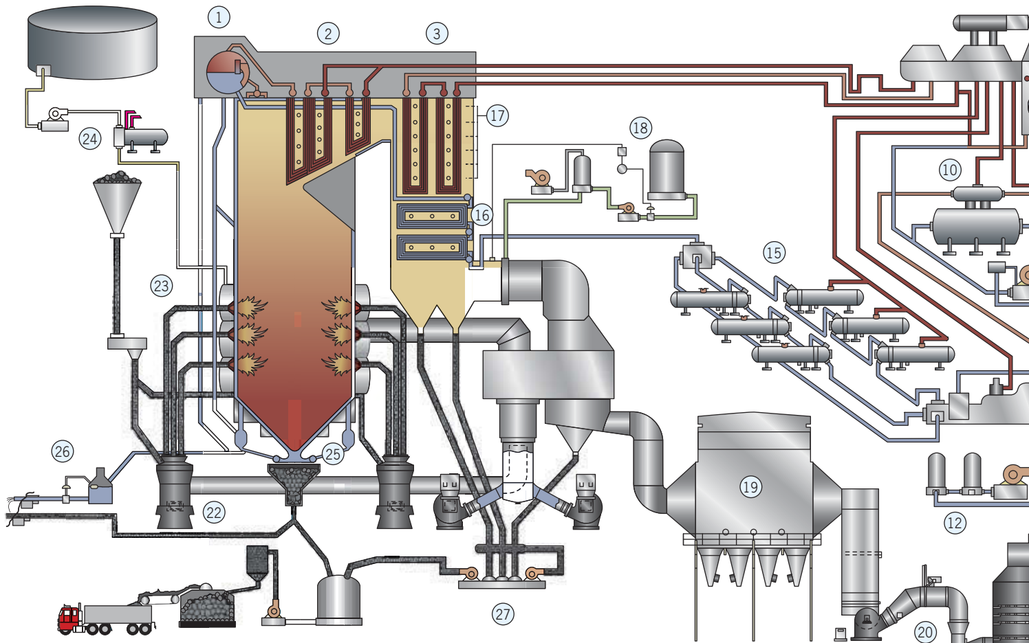
Conventional Power Plant Application, Applicable Valves and Operational Systems
