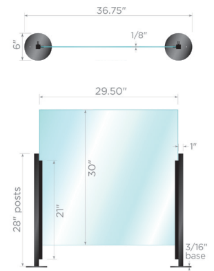
AC-SF-3030-SHIELD-BK 30"h x 30"w 6"w x 3/16"d base
