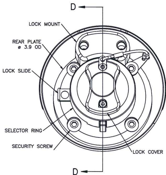
REAR PLATE ASSEMBLY
