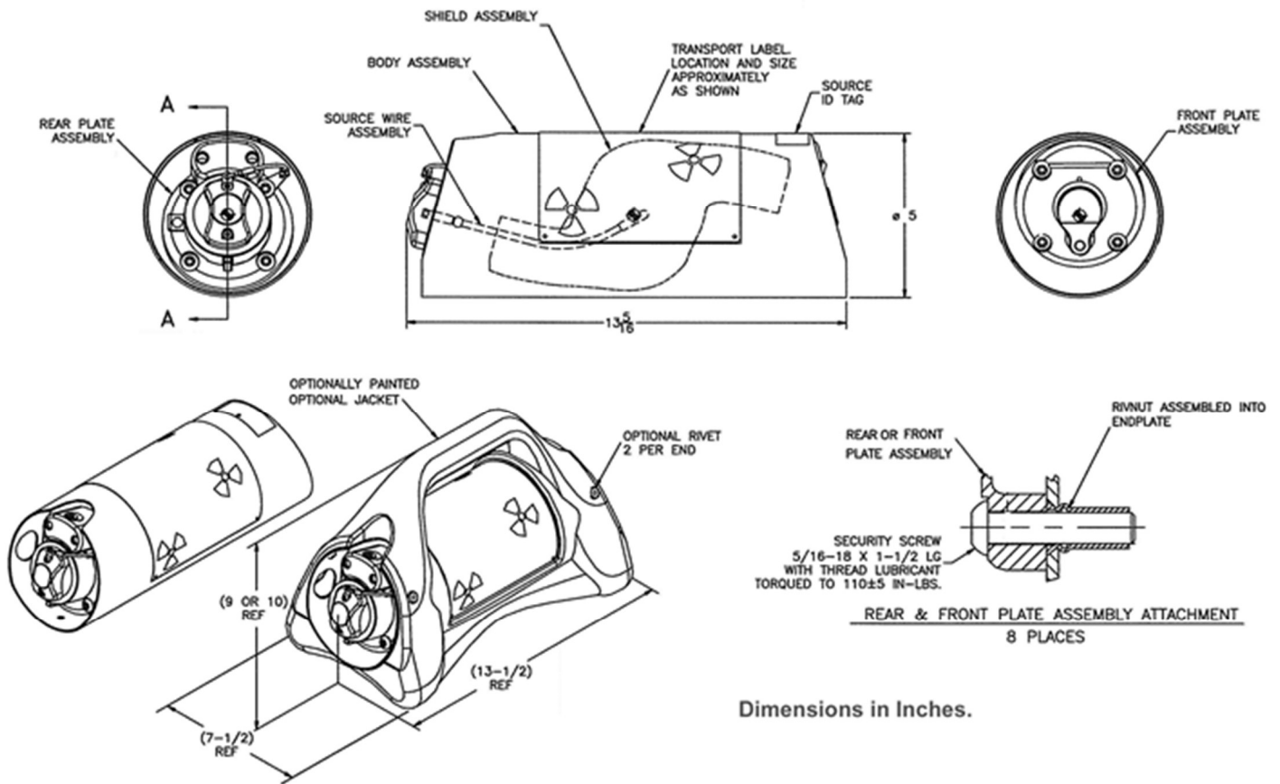
TRANSPORT PACKAGE WITHOUT & WITH OPTIONAL JACKET
