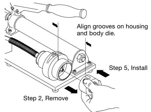
Fig. 2 Body Die Removal / Installation
