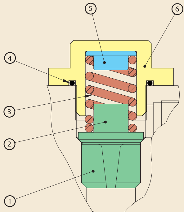
Preset Relief Valve Assembly
