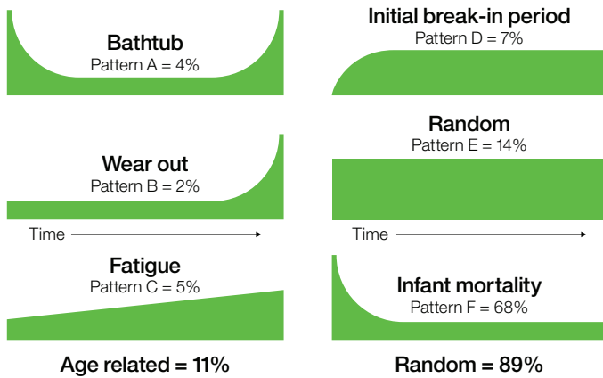
Figure 1: Failure curve models
