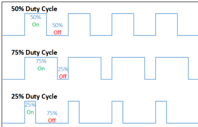
Figure 1. Pulse Width Modulation techniques break electrical current into a series of on-off sequences (Courtesy of Thewrightstuff, Wikipedia)
