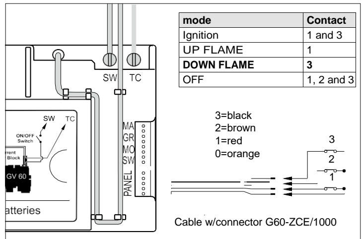
Figure 1: Wiring diagram and the operation sequence
