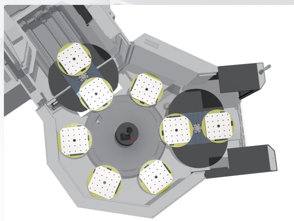
8 Pallets Operation
