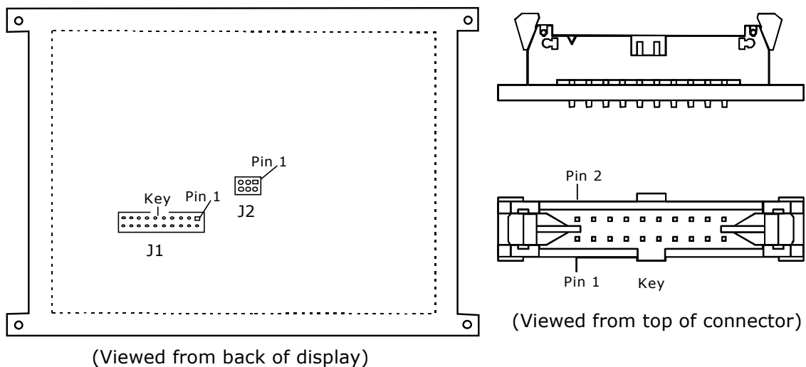
Figure 1. Data/power connector
