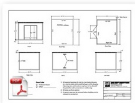
Model 10' x 12' Tapered Floor Plan
