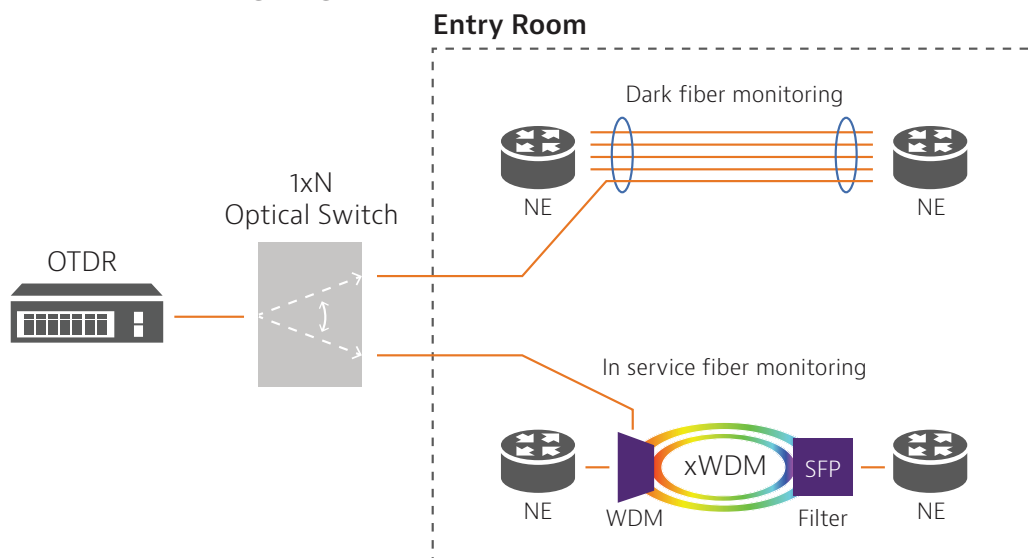
DCI Fiber Monitoring Diagram
