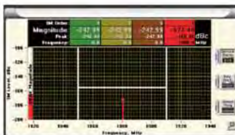
Dynamic PIM Test Results
