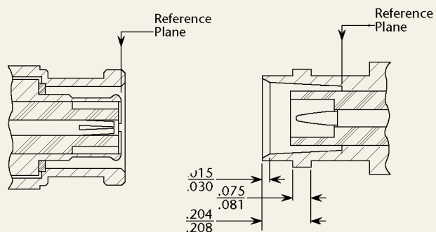
Plug (male)
