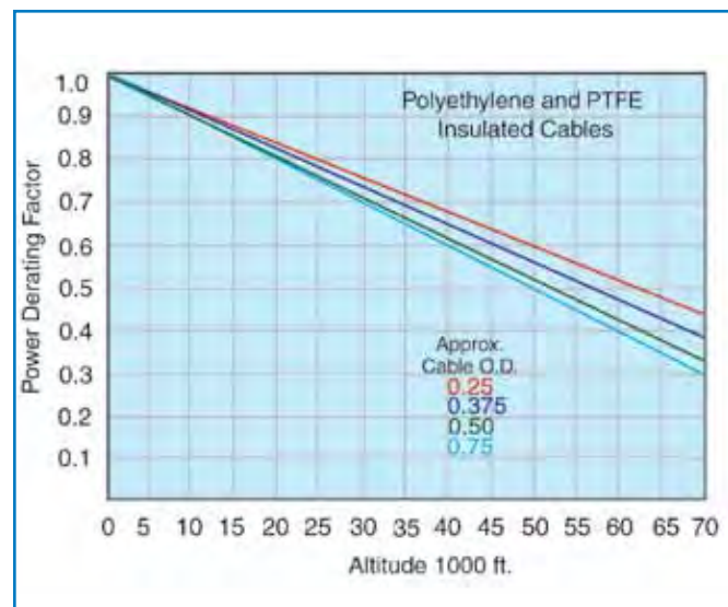
Power Altitude Correction Factor
