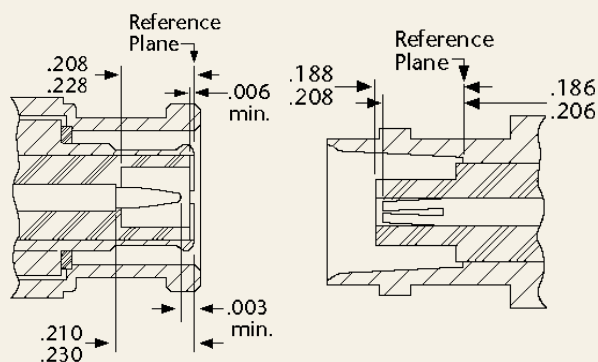
Plug (male)
