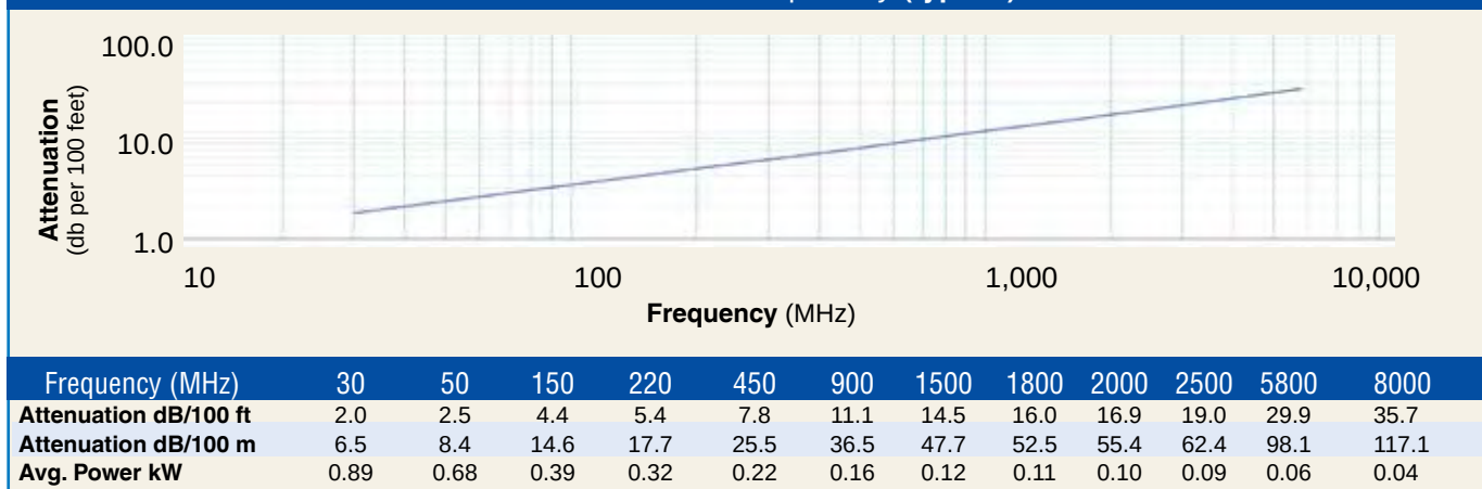
Attenuation vs. Frequency (typical)
