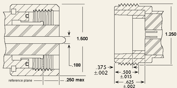
Plug (male)
