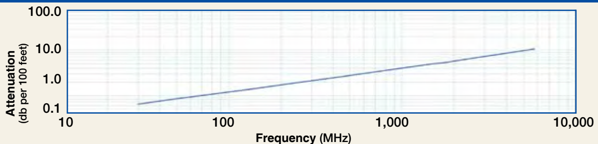
Attenuation vs. Frequency (typical)
