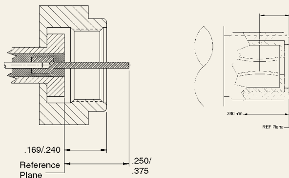
Plug (male)
