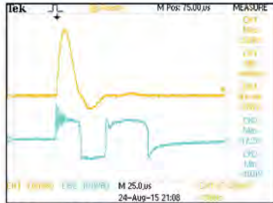
Surge Performance Data for the LP-DOE-1G
