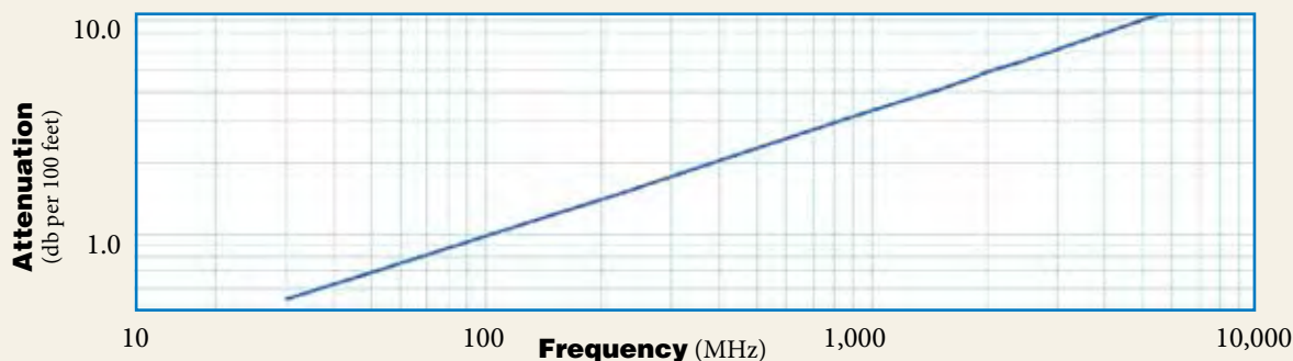
Attenuation vs. Frequency (typical)
