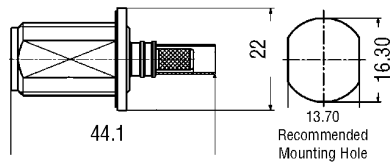
Type N Female Bulkhead 3190-2430
