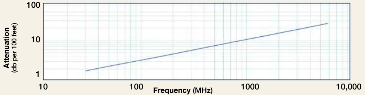
Attenuation vs. Frequency (typical)
