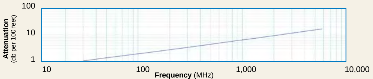
Attenuation vs. Frequency (typical)
