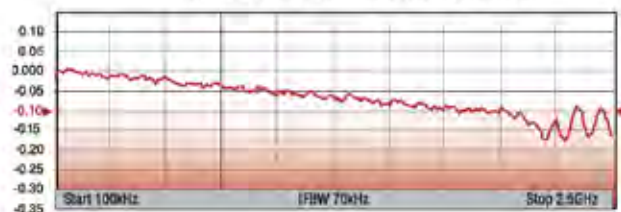
S21 TYPICAL INSERTION LOSS (dB)
