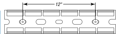
Minimum mounting rivet distance for ducts less than 1/2" wide.
