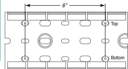
Minimum mounting rivet distance for ducts greater than 2/2" wide. Installed top and bottom.
