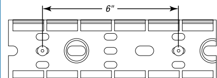
Minimum mounting rivet distance for ducts 1/2" to 2/2" wide.
