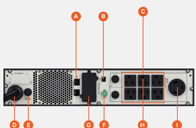
PSI5-3000RT120LI
