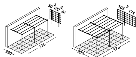
extension L 186
