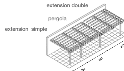
extension L 186
