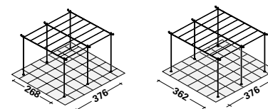
extension L 186
