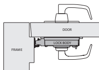
#2 STRIKE for single door out-swing PRODUCT NO. 2890-602
