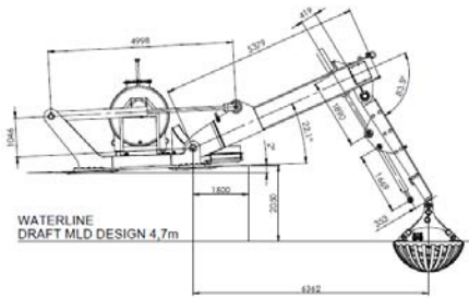
MAX. REACH
