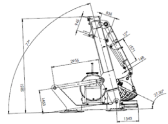
DECK POSITION
