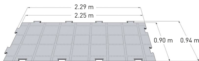
Dimensions ProPlay®-Sport sheet
