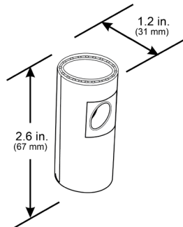
SU-5E Sensor Carrier
