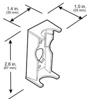
SU-5E Mounting Bracket
