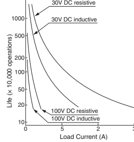
DC Load (RY2/4)
