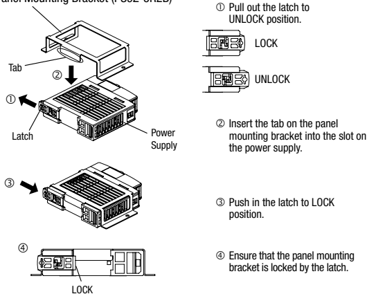
Panel Mounting Bracket (PS9Z-5R2B)
