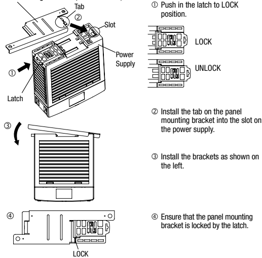
Panel Mounting Bracket (PS9Z-5R1□)
